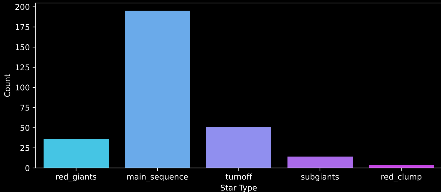
GALAH DR4 Field: [6930] Count plot of Star Type
