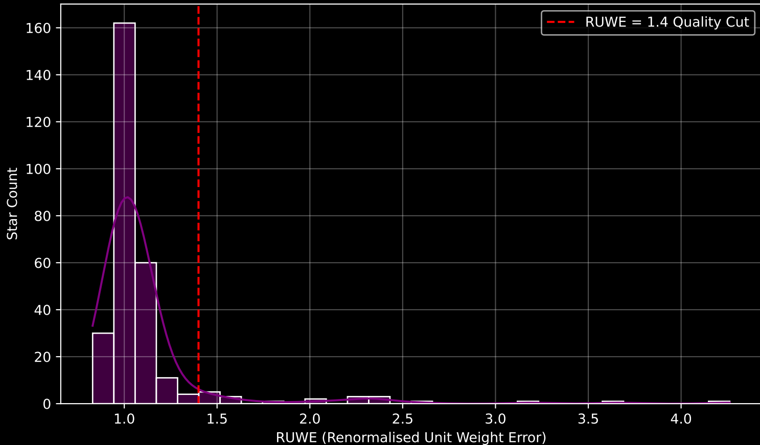
GALAH DR4 Field [6930] RUWE Distribution (n= 288)
