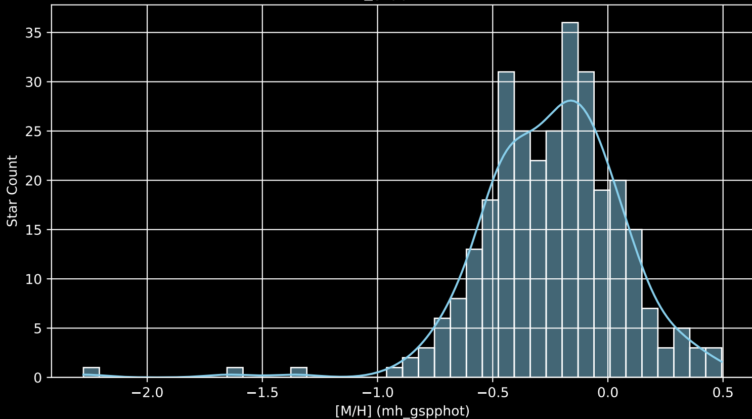
GALAH DR4 Field: [6930] [M/H] (mh_gspphot) (n= 299)
