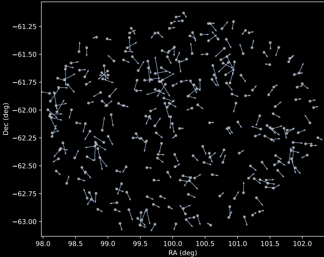
GALAH DR4 Cluster 1 Proper Motion Vectors (n=277)
