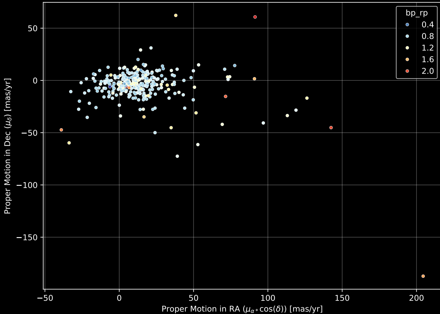
GALAH DR4 Field: [6930] Proper Motion Diagram (n= 300)
